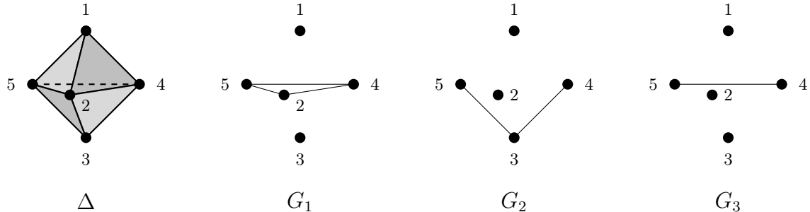
Figure 4: A bipyramid \Delta and its upper links G_1, G_2, G_3 .
