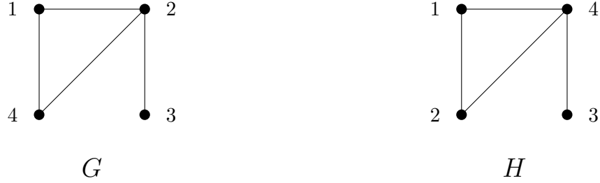
Figure 2: Two graphs G and H
