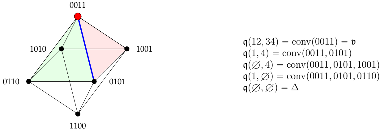
FIGURE 5. Locality for the hypersimplex \Delta_{2,4} .
