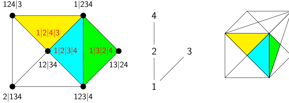
FIGURE 1. The normal fan of the cone in Example 2.6.
