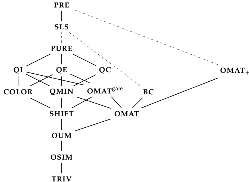
FIGURE 2. The hierarchy of Hopf classes of prefix-pure complexes. Solid lines indicate inclusions known to be strict; dashed lines indicate possible equalities. All classes are described in §§3.1–3.2, except \text{OMAT}_+ , which will be described in §5.3.
