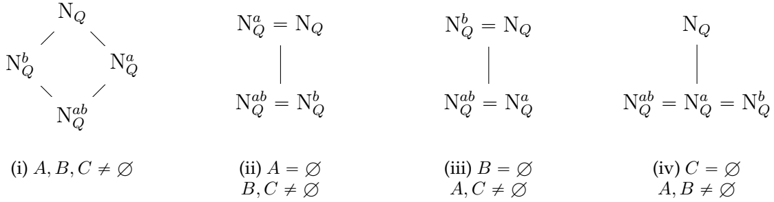
FIGURE 6. Possibilities for the interval [N_Q^{ab}, N_Q] .
