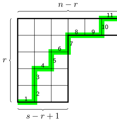
FIGURE 1. The panhandle matroid \text{Pan}_{5,7,11} as a lattice matroid. The lattice path shown in green gives rise to the basis \{2, 3, 5, 7, 10\} .
